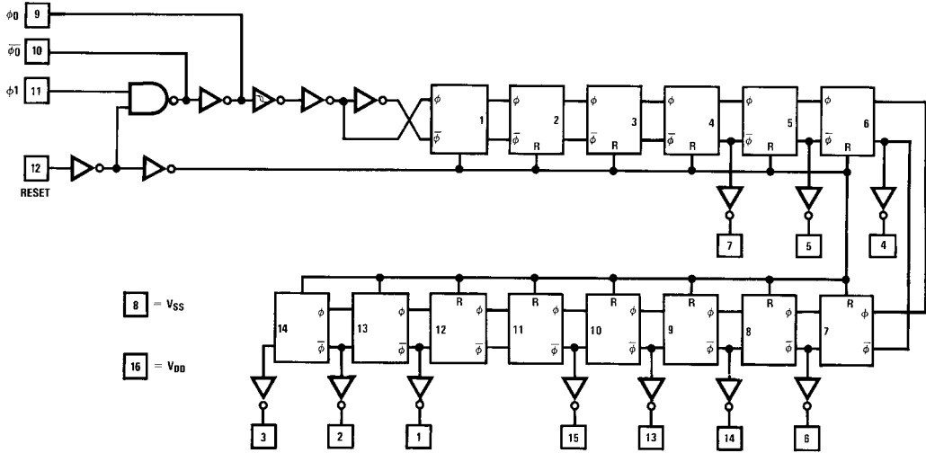
CD4060BC
