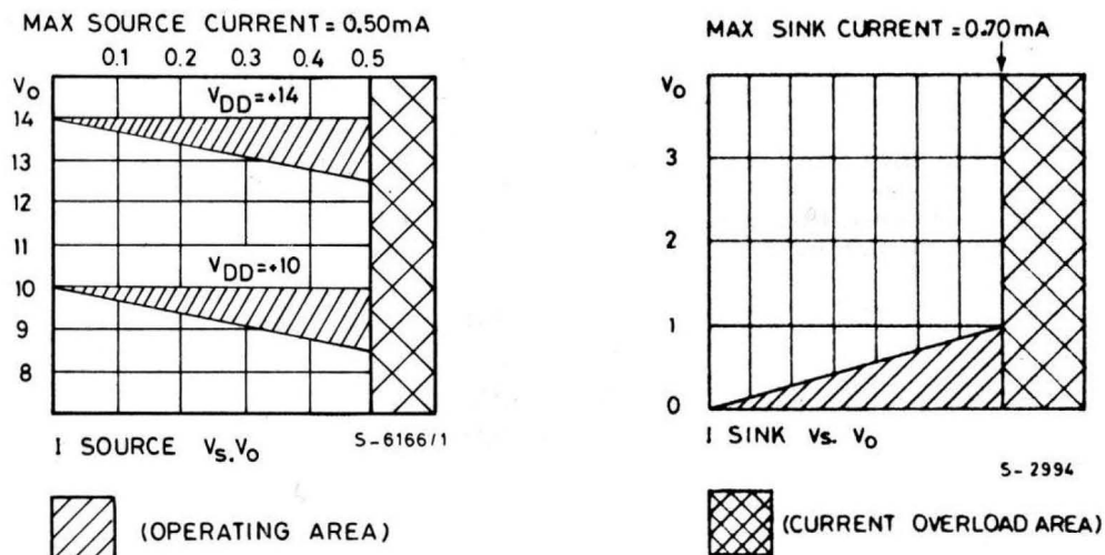
Fig. 2 - Output signal d.c. loading
