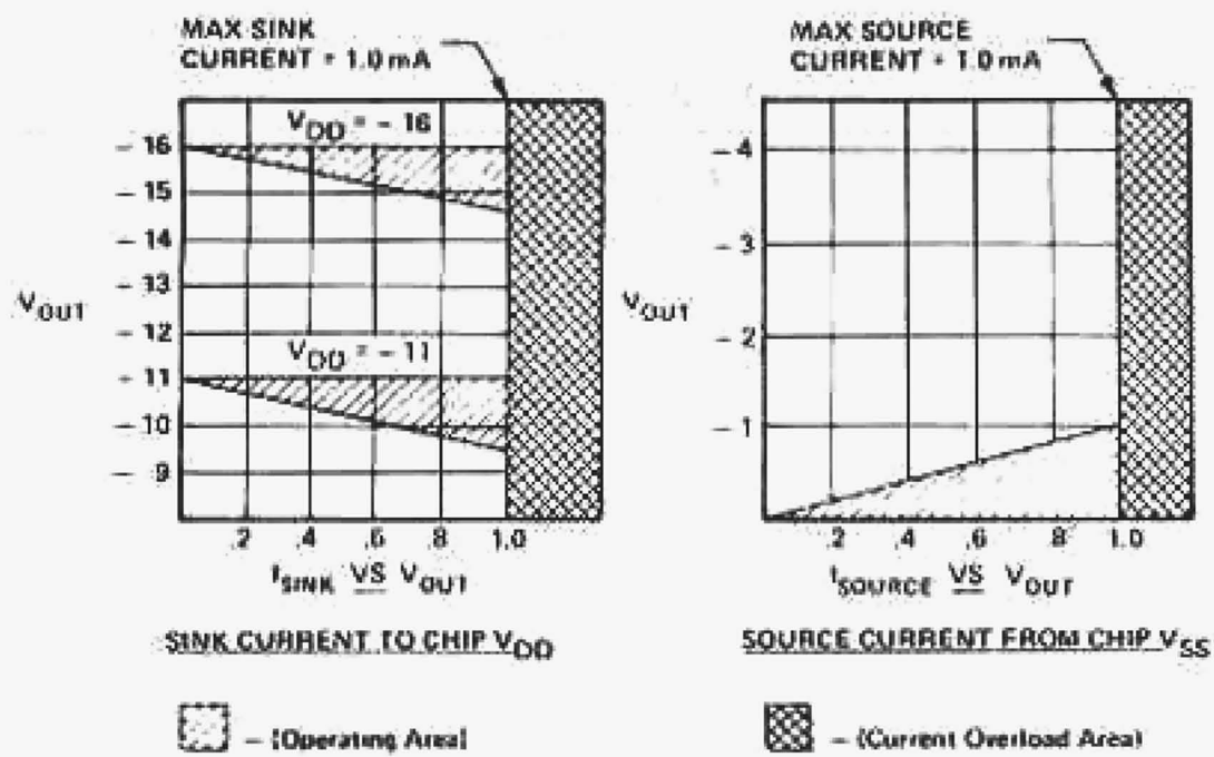
Figure 2. Output Signal DC Loading
