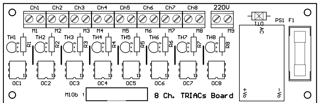
TRIACs Board Silkscreen (140 x 45 mm.)
