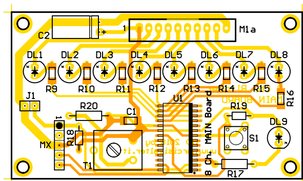
MAIN Board Silk Screen (25 x 43 mm)
