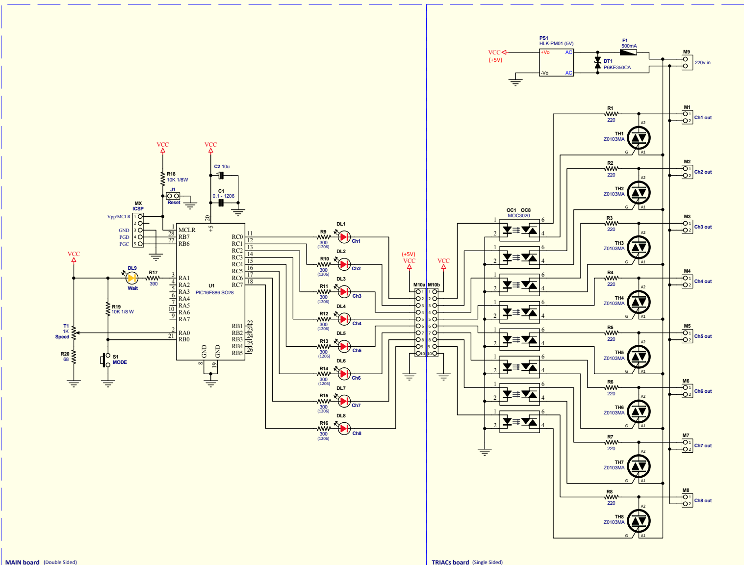
MAIN board (Double Sided)
