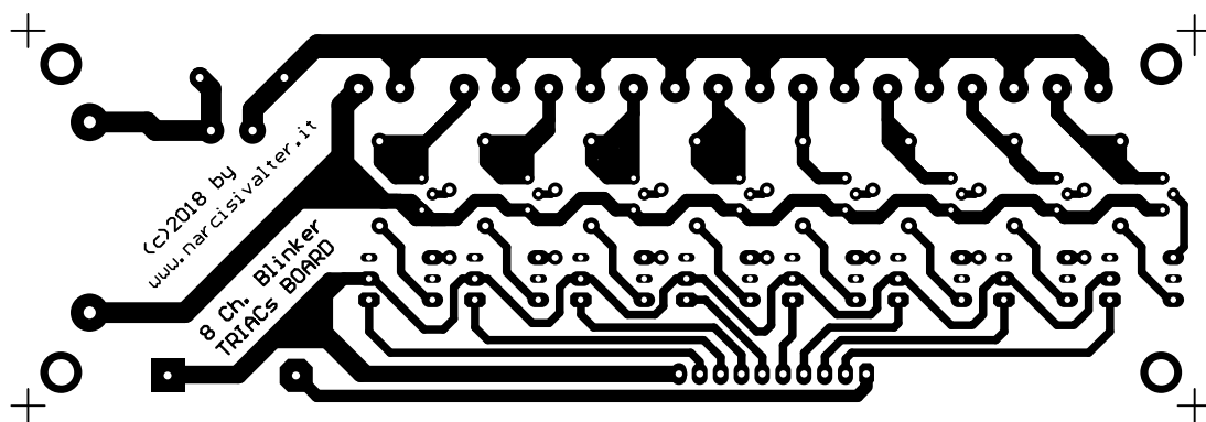
TRIACs Board (Bottom Layer 140 x 45 mm.)
