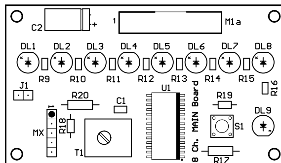
MAIN Board Silkscreen (75 x 43 mm.)
